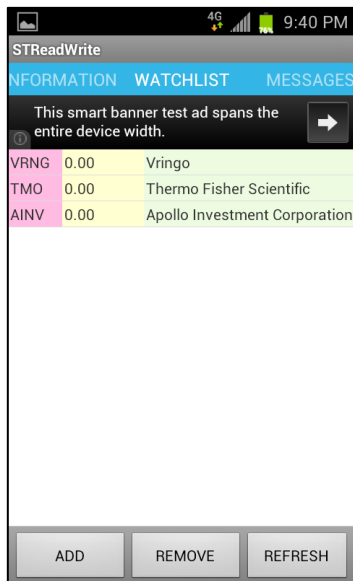
Watchlist View.
