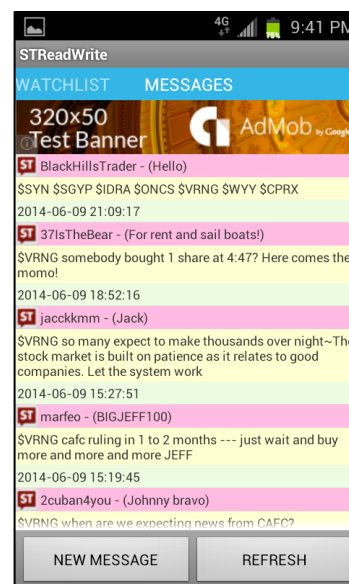
Messages View.
